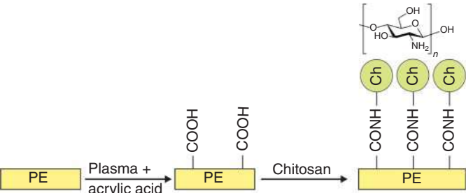
Figure 2.25 The scheme of chitosan immobilization on the polymer surface.
