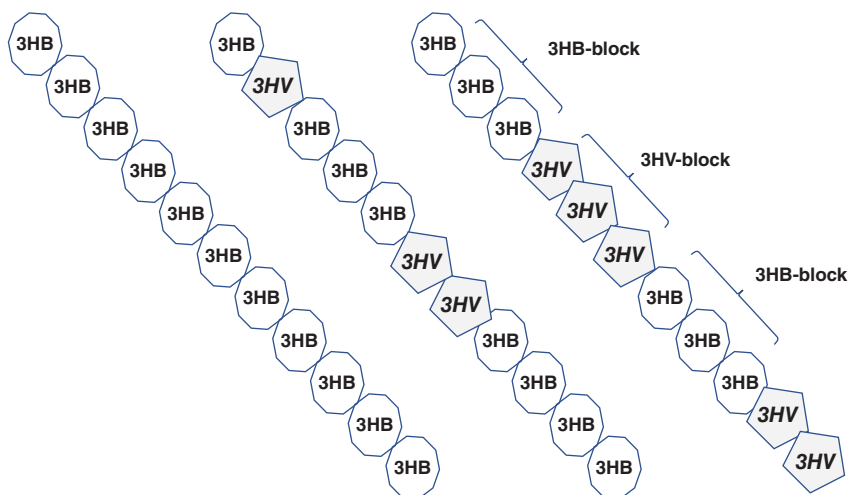
Figure 1.11 Schematic of PHA homopolymer (left polymer chain; the polyester represents PHB), poly(3HB-co-3HV) with random distribution (middle polymer chain), and blocky structured poly(3HB-b-3HV). Spheres represent 3HB building blocks, pentagons 3HV.
