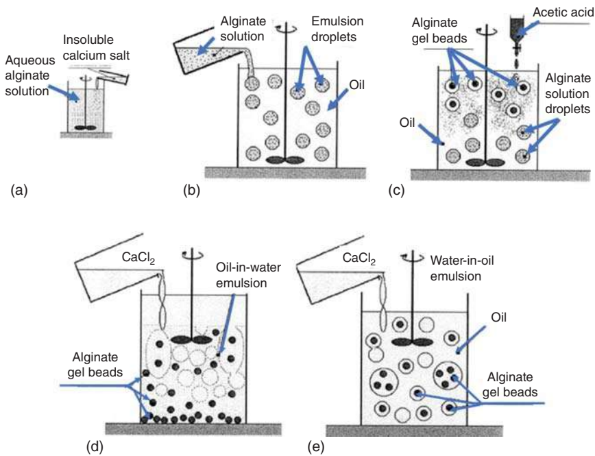
Figure 16.6 Different stages of the preparation of alginate beads by emulsification: internal gelation method. Source: Poncelet et al. [63]/with permission from Elsevier.
