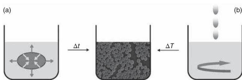
Figure 9.1 Schematic presentation of nanoprecipitation methods applying dialysis (a) and the dropping technique under stirring (b). Source: Hornig et al. [12]/with permission of the Royal Society of Chemistry.
