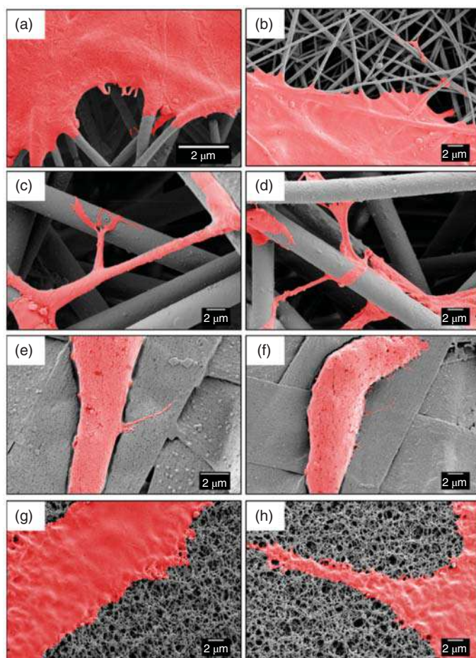
Figure 15.2 SEM micrographs showing cell attachment to a different type of scaffold, after three days: (a, b) nanofibers, (c, d) microfibers, (e, f) ribbons, and (g, h) film; cells are colored in red. Source: Ura et al. [46]/MDPI/CC BY 4.0.
