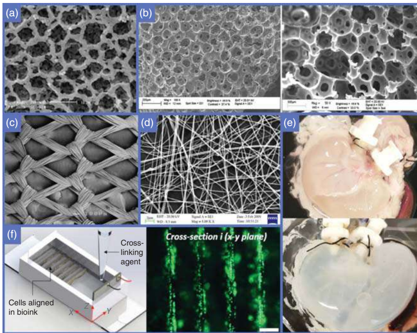
Figure 10.2 Scaffold fabrication approaches without the aid of computer-aided design and manufacturing. (a) A scanning electron micrograph of PVDF scaffolds prepared by phase separation. Source: From Abzan et al. [56]/with permission of Elsevier. (b) SEM images of PVA scaffolds prepared by using classical gas foaming (right) or microfluidic gas foaming (left). Source: Reproduced from Colosi et al. [57]/with permission of American Chemical Society. (c) Woven PLGA scaffold. Source: Reproduced from Chen et al. [58]/with permission of Elsevier. (d) Scanning electron micrograph of electrospun polyethylene oxide fibers. Source: Reproduced from Bhardwaj and Kundu [59]/with permission of Elsevier. (e) Scaffold preparation using decellularization of a rat stomach before (upper image) and after (lower image) detergent enzymatic treatment. Source: Reproduced from Zambaiti et al. [60]/with permission of Springer Nature. (f) Scaffold fabrication using standing waves with ultrasound patterning of bioink. On the right, a microscopic image is shown using a live/dead assay with living cells colored green. Source: Reproduced from Chansoria et al. [61]/with permission IOP Publishing Ltd/reproduced from Zambaiti et al. [60]/with permission of Springer Nature.
