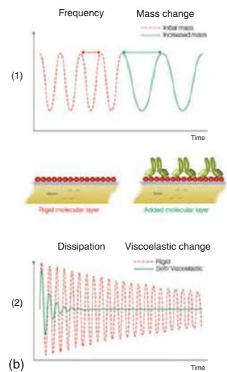
Figure 4.11 (a) A schematic representation of the QCM device and its key elements, (b) examples of frequency and dissipation recordings.
