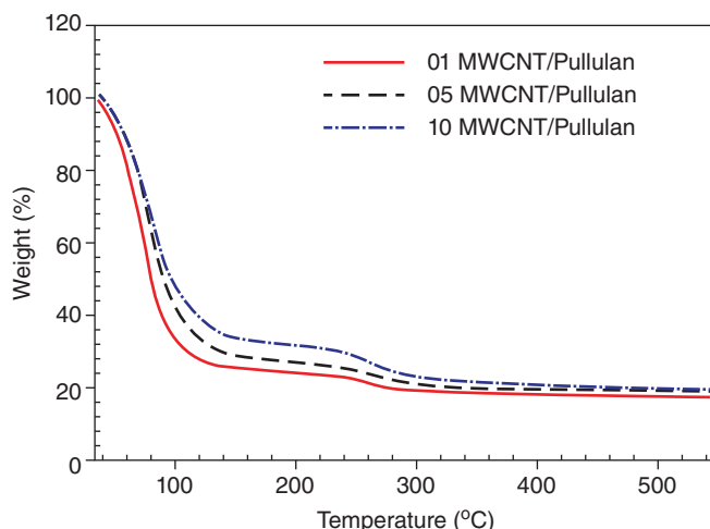
Figure 3.7 Thermogravimetric analysis of pullulan/MWCNT hydrogels. Source: Saeaehe et al. [20]/with permission of Elsevier.
