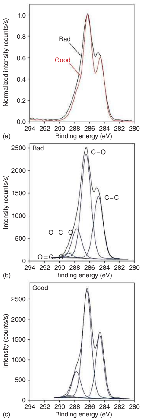
Figure 2.14 (a) A comparison of the two selected C1s spectra from Figure 2.13 as an example of a broadening of the C1s spectra because of charging as a consequence of the good or bad selection of surface neutralization conditions. (b) and (c) Deconvolution of these two selected spectra.
