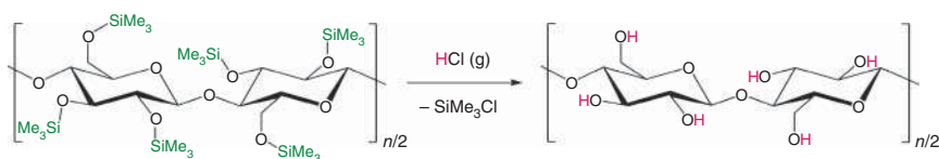
Figure 6.3 Regeneration of TMSC to cellulose by exposure to HCl vapor.
