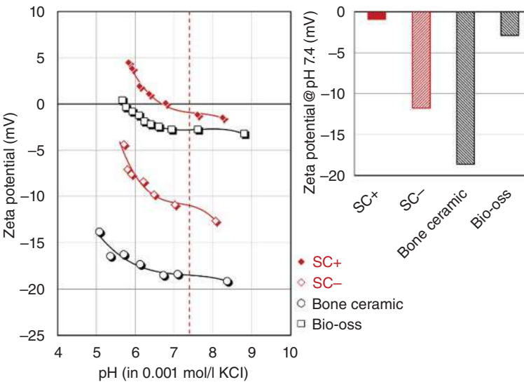
Figure 4.9 Comparison of the pH dependence of the zeta potential for a series of commercial bone fillers BoneCeramic® (Straumann USA LLC), Bio-Oss® (Geistlich Pharma AG), and Synergoss® (Nobil Bio Ricerche srl) with (SC+) and without collagen coating (SC-). The zeta potential at the physiological pH 7.4 indicated by the dashed line is shown in the separate chart. Source: Adapted from Iviglia et al. [80].
