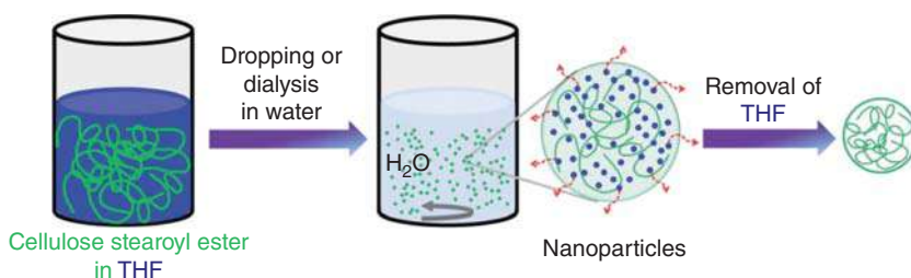
Figure 9.3 Schematic illustration for the nanoprecipitation of cellulose stearoyl ester. Source: Geissler et al. [19]/with permission of the Royal Society of Chemistry.
