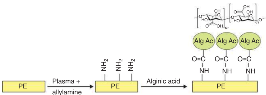
Figure 2.23 Scheme of alginic acid immobilization on the polymer surface.
