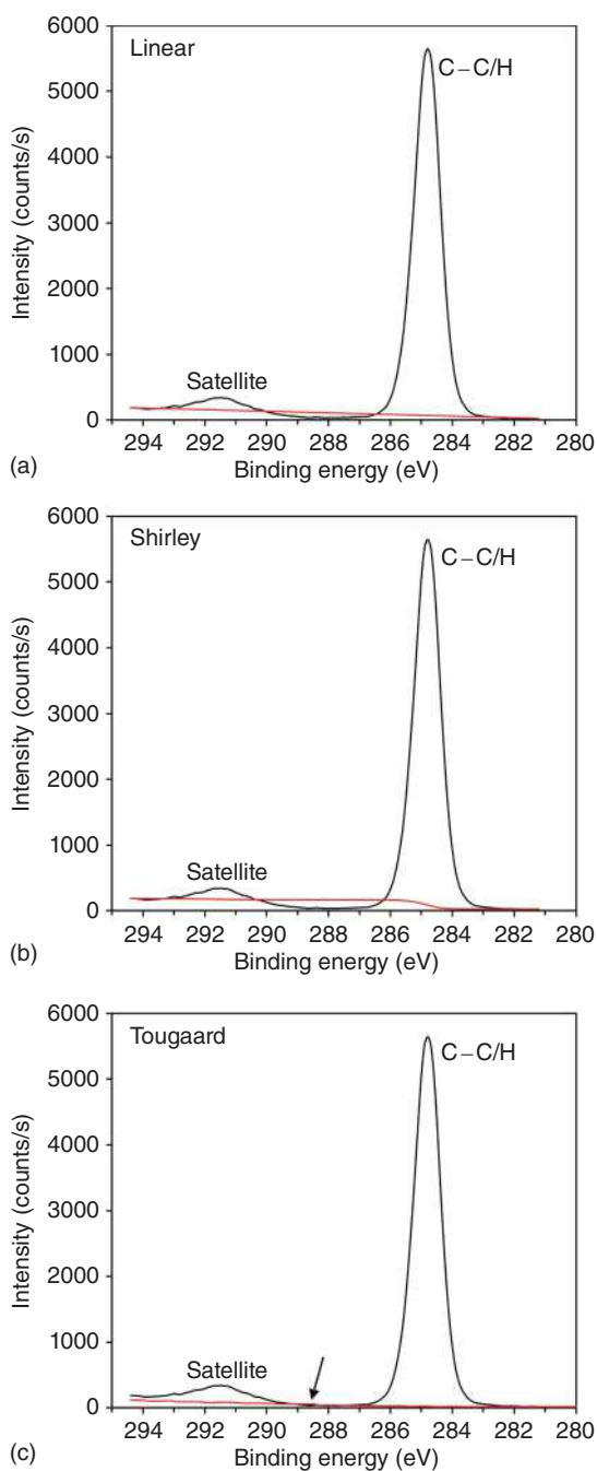
Figure 2.15 Some examples of using different types of background subtraction for C1s peak of polystyrene: (a) linear, (b) Shirley, and (c) Tougaard subtraction. An arrow in Figure 2.15c indicates a small portion of the spectrum, where the background cuts the spectrum. In the case of figures (a) and (b), the part of the cutoff spectrum is much larger.
