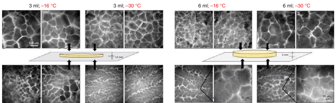
Figure 13.8 Fluorescent microscopy images depicting FITC-labeled gelatin component of polypropylene mesh–gelatin composites. Composites contain two different volumes (3 and 6 ml) of 10% gelatin solution and are exposed to different, unidirectional freezing end temperatures ( -16 and -30 °C). Both the air-exposed side and cooling plate-exposed side are presented, referring to the relative position of composite surface with freezing plate surface. Source: From Gorgieva [54]/with permission of American Chemical Society.
