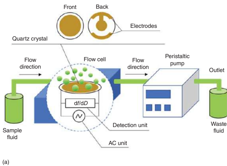
Figure 4.11 (a) A schematic representation of the QCM device and its key elements, (b) examples of frequency and dissipation recordings.
