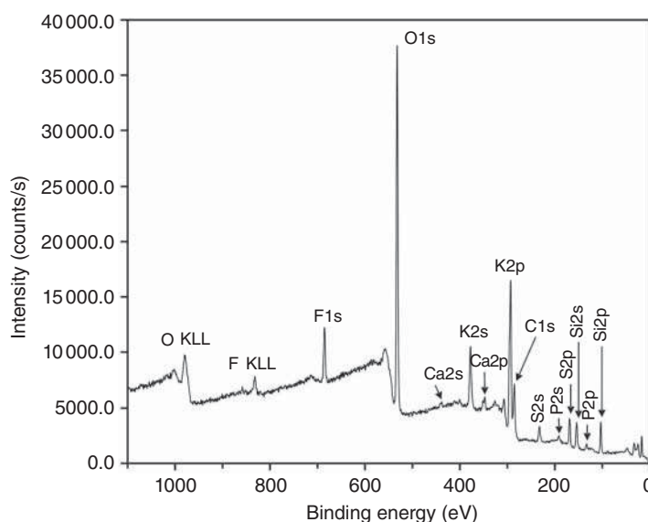
Figure 2.32 The XPS survey spectrum of chestnut honey after cold plasma ashing in oxygen afterglow.
