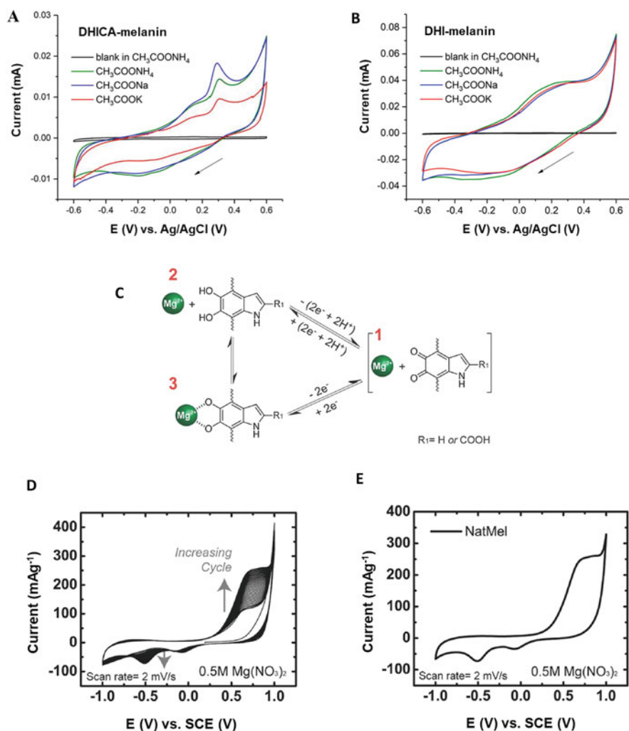
Fig. 5 Electrochemical behavior of eumelanin. DHICA-melanin (a) and DHI-melanin (b) in the presence of monovalent ions, \nu = 5 \text{ mV/s} , acid buffers. Adapted from ref. (Xu et al. 2017). (c) Mechanism proposed for the interaction/cooordination of \text{Mg}^{2+} ions in the catechol groups in Sepia melanin during voltammetry cycles. States 1 and 3 represent the melanin in the direction of oxidation and reduction states, respectively. State 2 represents an intermediate state of a catechol group before forming a coordination bonding. (d) and (e) represent the cyclic voltammeteries of Sepia melanin in the presence of an electrolyte based on \text{Mg}^{2+} ions, 0.5 \text{ M Mg(NO}_3)_2 . Adapted from ref. (Kim et al. 2014)
