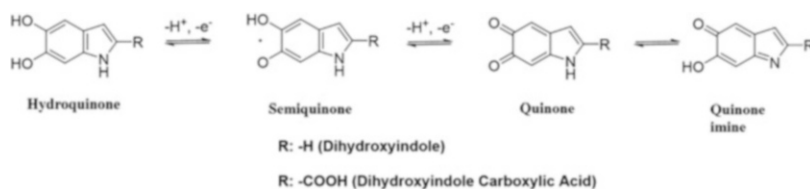
Fig. 5 Different redox forms of melanin monomeric structures: R = H (DHI) or COOH (DHICA) (Realí et al. 2021)
