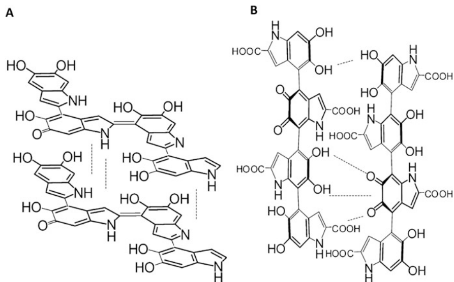
Fig. 3 Supramolecular structures of DHI- and DHICA-melanins. (a) DHI melanin represented as planar oligomeric scaffolds, (b) DHICA melanin is made up of twisted linear oligomer structures featuring atropisomerism. Adapted from ref. (d'Ischia et al. 2014)
