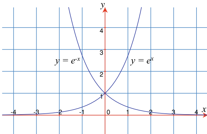
Fig. 16.8 Graphs of y = e^x and y = e^{-x}
