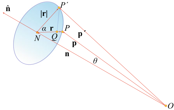
Fig. 15.11 The geometry associated with rotating a point about an arbitrary axis
