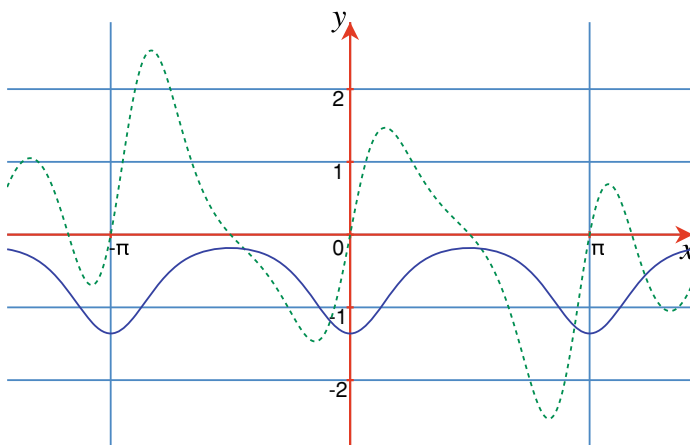
Fig. 17.26 The graphs of y = 2e^{\cos 2x} \sin x \cos x (dashed) and y = -\frac{1}{2}e^{\cos 2x}
