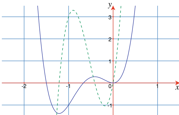
Fig. 16.5 Graph of y = (3x^2 + 2x)(2x^2 + 3x) and its derivative, \frac{dy}{dx} = 24x^3 + 39x^2 + 12x (dashed)
