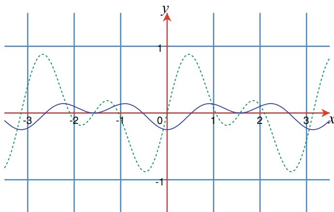
Fig. 17.7 The graphs of y = \sin(3x) \cdot \cos x (dashed) and y = -\frac{1}{8} \cos(4x) - \frac{1}{4} \cos(2x)
