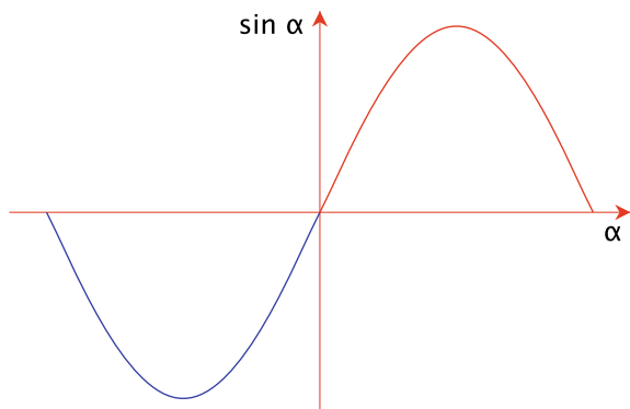
Fig. 4.6 The sine function is an odd function
