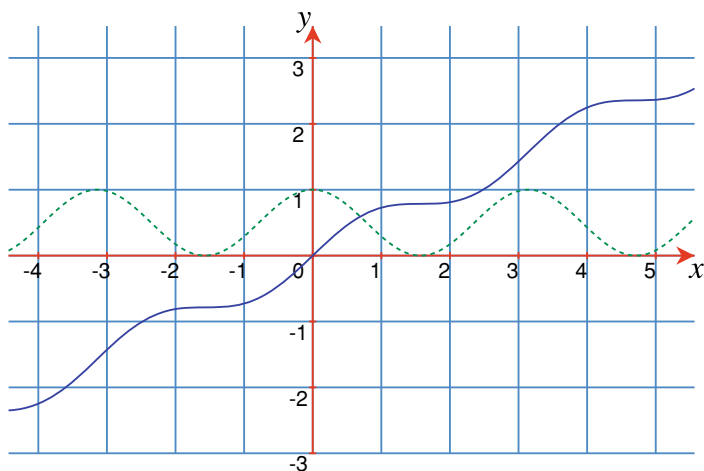
Fig. 17.5 The graphs of y = \cos^2 x (dashed) and y = \frac{1}{4} \sin(2x) + \frac{1}{2}x
