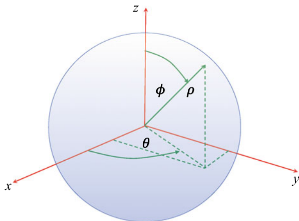
Fig. 19.25 Spherical Polar Coordinates
