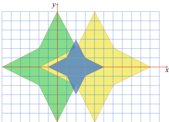
Fig. 14.2 A translate transform followed by a scale transform
