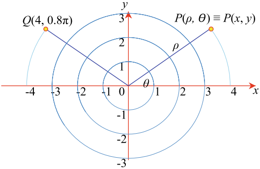
Fig. 10.7 2D polar coordinates
