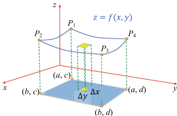
Fig. 19.17 A surface created by z = f(x, y)
