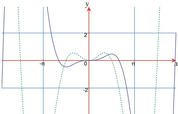
Fig. 17.15 The graphs of y = x^2 \cos x (dashed) and y = x^2 \sin x + 2x \cos x - 2 \sin x
