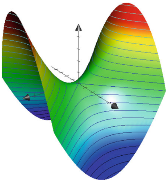
Fig. 16.20 Surface of z = 2.5x^2 - 2.5y^2 using a right-handed axial system with a vertical z -axis
