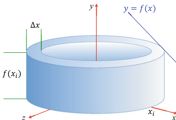
Fig. 19.12 Dimensions for one concentric shell
