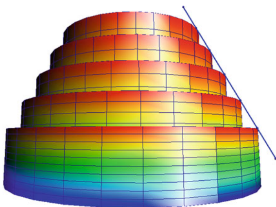
Fig. 19.11 A series of concentric shells
