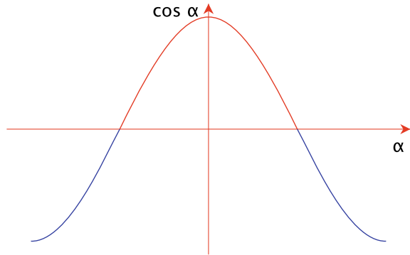
Fig. 4.7 The cosine function is an even function
