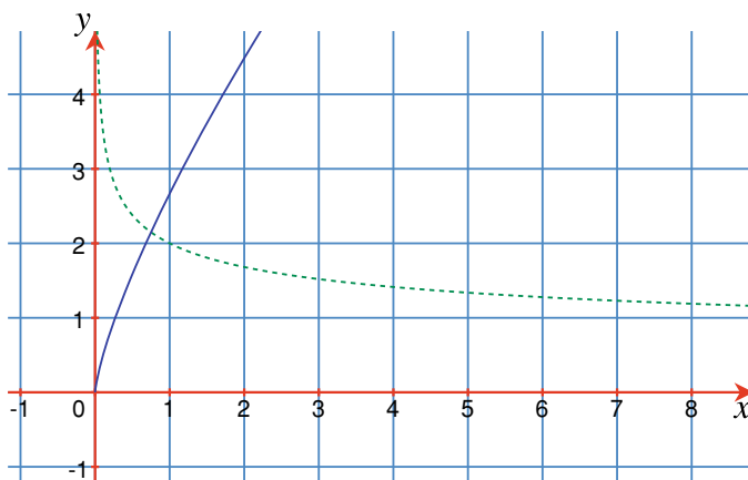
Fig. 17.8 The graphs of y = 2/\sqrt[4]{x} (dashed) and y = 8x^{\frac{3}{4}}/3
