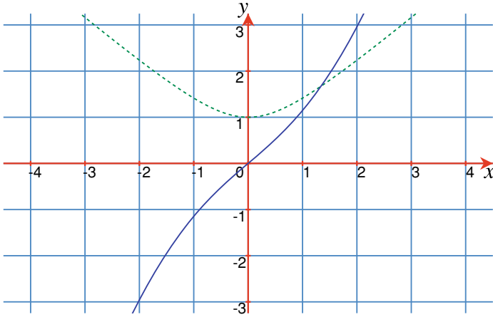
Fig. 17.17 The graphs of y = \sqrt{1+x^2} (dashed) and y = \frac{1}{2}x\sqrt{1+x^2} + \frac{1}{2}\operatorname{arsinh}x
