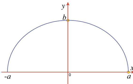
Fig. 19.7 Part of an ellipse used to form an ellipsoid
