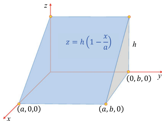
Fig. 19.19 A prism
