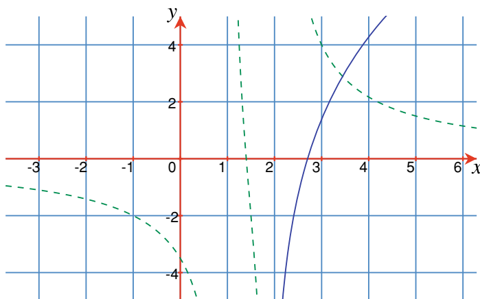
Fig. 17.21 The graphs of y = (5x - 7)/((x - 1)(x - 2)) (dashed) and y = 2 \ln(x - 1) + 3 \ln(x - 2)
