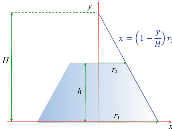
Fig. 19.5 Computing the volume of a right conical frustum
