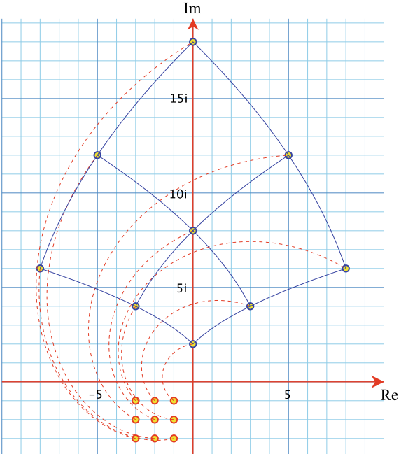
Fig. 13.15 The trajectories of nine complex numbers in the third quadrant, when squared
