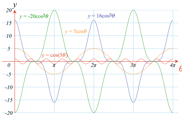
Fig. 13.19 \cos(5\theta) = 16\cos^5\theta - 20\cos^3\theta + 5\cos\theta
