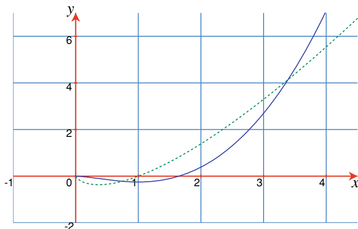
Fig. 17.16 The graphs of y = x \ln x (dashed) and y = \frac{1}{2}x^2 \ln x - \frac{1}{4}x^2
