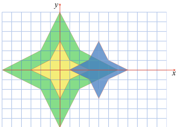
Fig. 14.1 A scale transform followed by a translate transform
