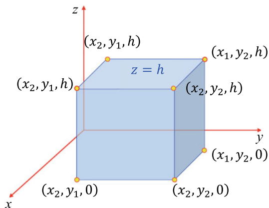
Fig. 19.18 A rectangular box
