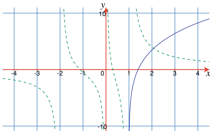
Fig. 17.29 The graphs of y = (6x^2 + 5x - 2)/(x^3 + x^2 - 2x) (dashed) and y = \ln x + 2 \ln(x + 2) + 3 \ln(x - 1)
