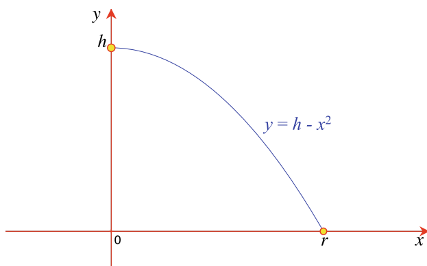
Fig. 19.16 The geometry used to create a paraboloid
