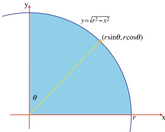
Fig. 18.10 Area under the graph is \int_0^r \sqrt{r^2 - x^2} dx
