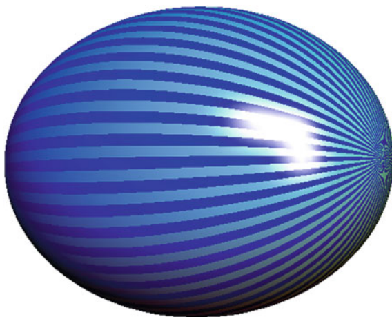
Fig. 19.8 An ellipsoid
