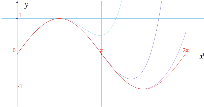
Fig. 13.8 The sine power series for different number of terms
