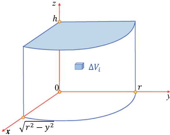
Fig. 19.24 The first quadrant of a circular arc
