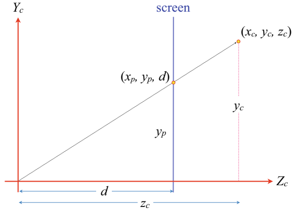
Fig. 15.16 A side view of the camera's axial system
