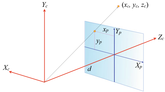
Fig. 15.14 The axial system used for the perspective projection
