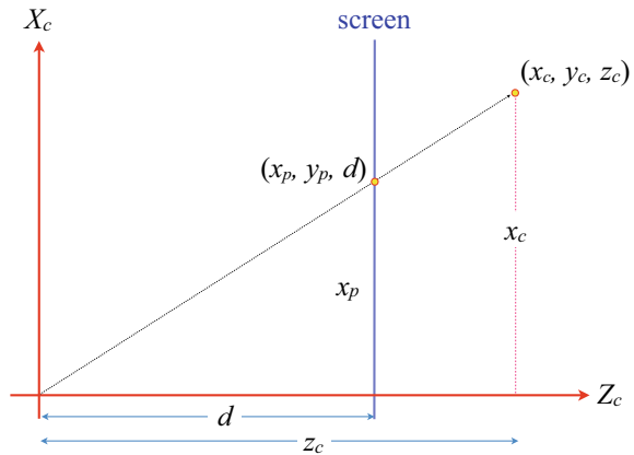
Fig. 15.15 A plan view of the camera's axial system
