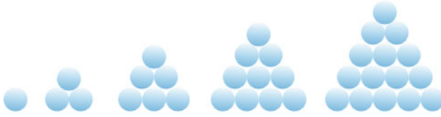
Fig. 2.3 First five triangular numbers
