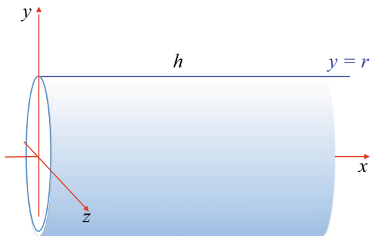
Fig. 19.2 Computing the volume of a cylinder
