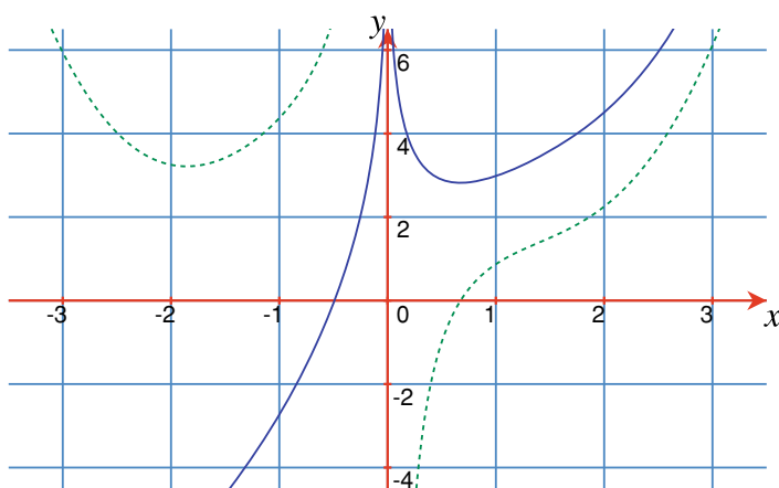
Fig. 17.13 The graphs of y = (4x^3 + x^2 - 8 + 12x \cos x)/4x (dashed) and y = x^3/3 + x^2/8 - 2 \ln |x| + 3 \sin x
