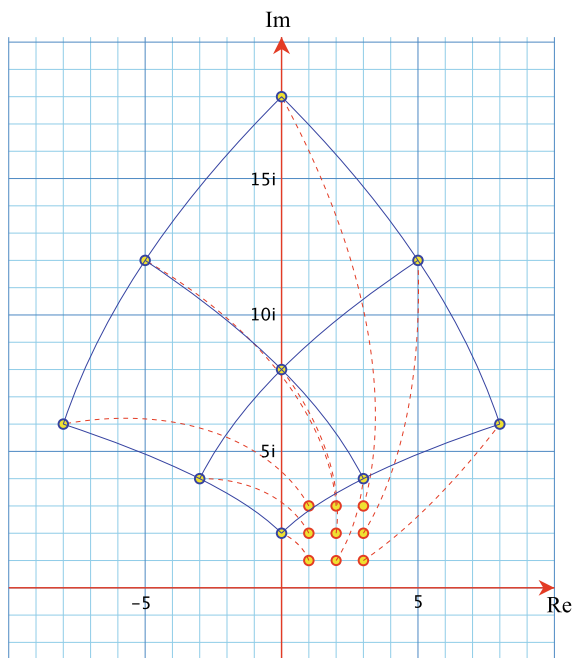
Fig. 13.13 The trajectories of nine complex numbers in the first quadrant, when squared
