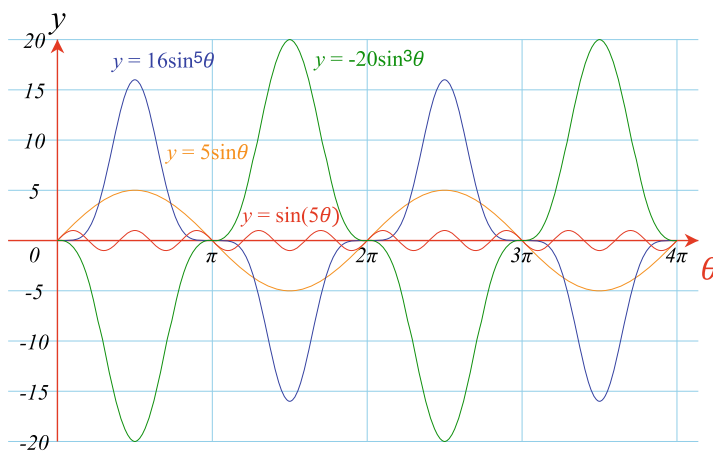
Fig. 13.20 \sin(5\theta) = 16\sin^5\theta - 20\sin^3\theta + 5\sin\theta
