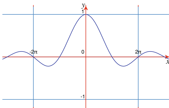
Fig. 17.2 Graph of y = (\sin x)/x
