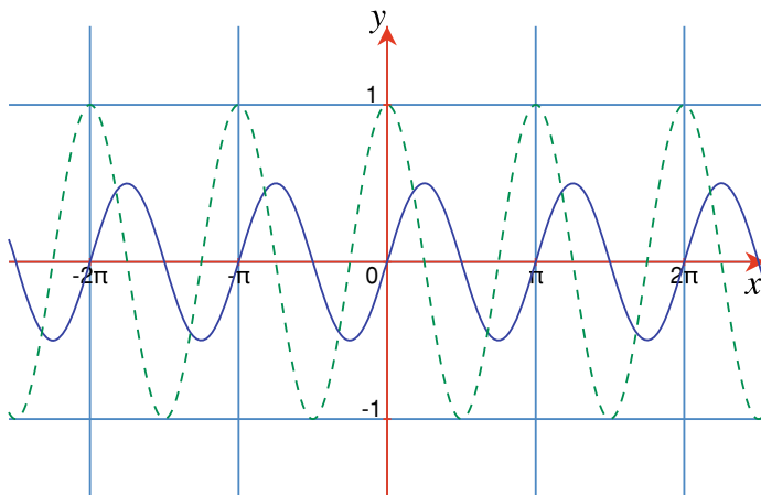
Fig. 16.6 Graph of y = \sin x \cos x and its derivative, \frac{dy}{dx} = \cos(2x) (dashed)
