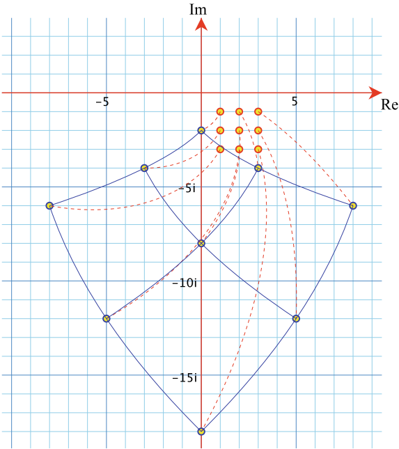
Fig. 13.16 The trajectories of nine complex numbers in the fourth quadrant, when squared
