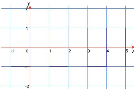
Fig. 17.1 A discontinuous square-wave function
