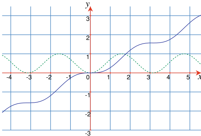
Fig. 17.4 The graphs of y = \sin^2 x (dashed) and y = \frac{1}{2}x - \frac{1}{4} \sin(2x)
