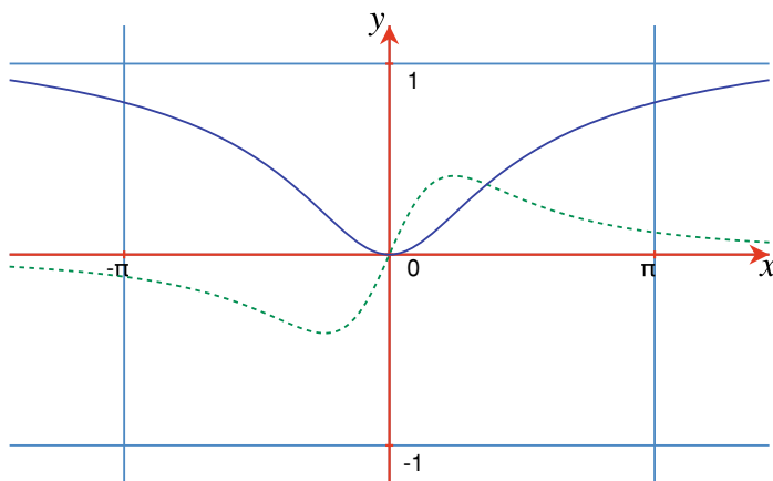
Fig. 17.11 The graphs of y = \arctan x / (1 + x^2) (dashed) and y = \frac{1}{2}(\arctan x)^2
