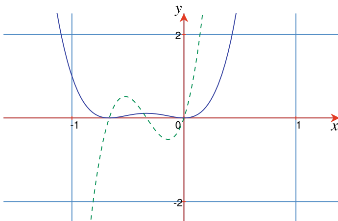
Fig. 16.3 Graph of y = (3x^2 + 2x)^2 and its derivative, \frac{dy}{dx} = 36x^3 + 36x^2 + 8x (dashed)
