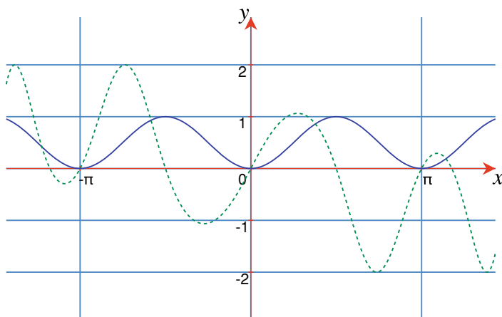
Fig. 17.19 The graphs of y = 2 \sin x \cdot \cos x (dashed) and y = \sin^2 x
