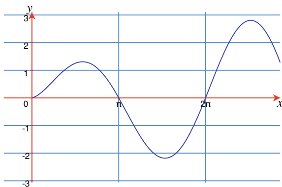
Fig. 17.3 Graph of y = \sqrt{x} \sin x
