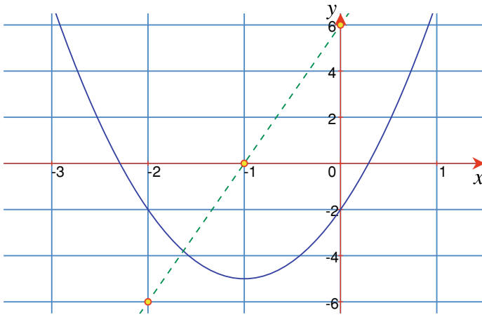
Fig. 16.19 A function containing a local minimum, and its first derivative (dashed)
