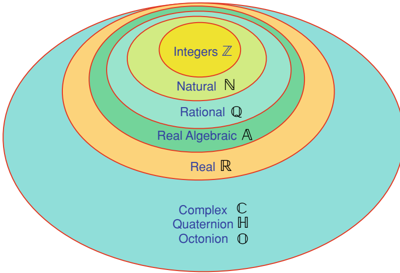
Fig. 2.2 The nested sets of numbers
