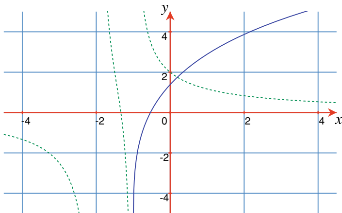
Fig. 17.20 The graphs of y = (3x + 4)/((x + 1)(x + 2)) (dashed) and y = \ln(x + 1) + 2 \ln(x + 2)
