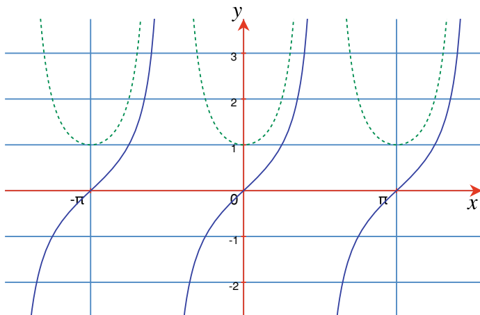
Fig. 16.11 Graph of y = \tan x and its derivative, \frac{dy}{dx} = 1 + \tan^2 x (dashed)
