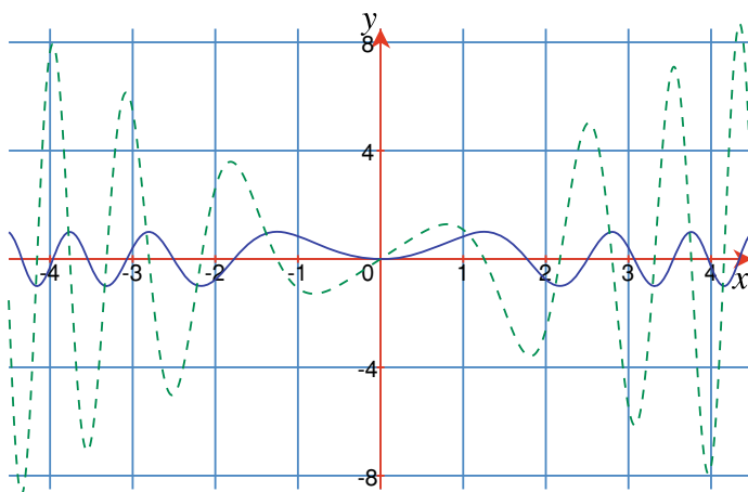
Fig. 16.4 Graph of y = \sin x^2 and its derivative, \frac{dy}{dx} = 2x \cos x^2 (dashed)
