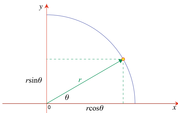
Fig. 19.15 The geometry used to create a hemisphere
