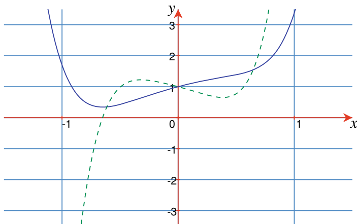
Fig. 16.2 Graph of y = 2x^6 + \sin x + \cos x and its derivative, \frac{dy}{dx} = 12x^5 + \cos x - \sin x (dashed)
