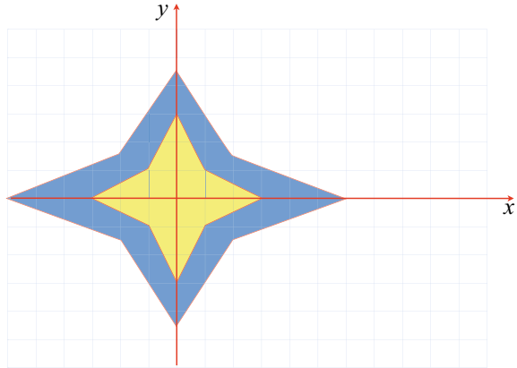
Fig. 15.2 Asymmetric scaling relative to the origin
