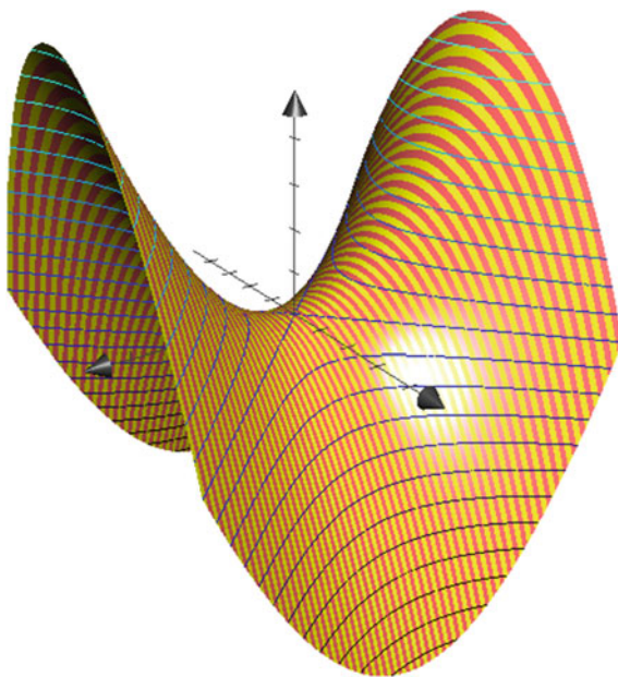
Fig. 16.22 \frac{\partial z}{\partial y} describes the slopes of these contour lines
