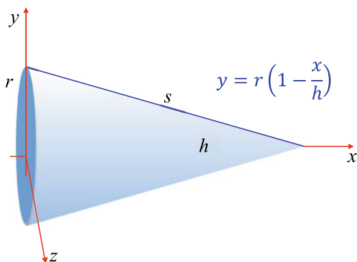
Fig. 19.4 Reversing the orientation of a right cone
