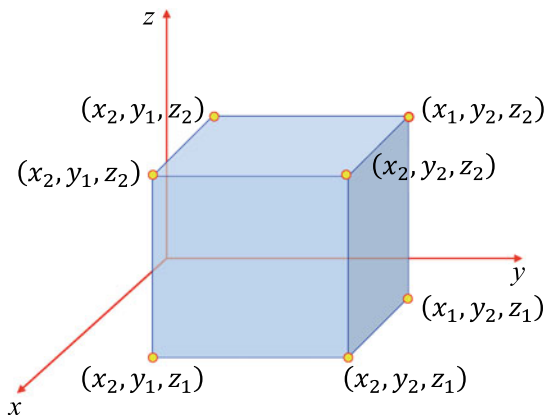
Fig. 19.23 Cartesian coordinates for a rectangular box
