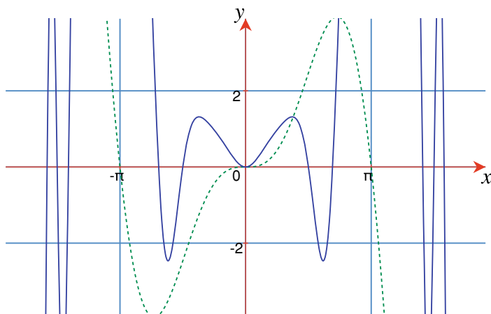
Fig. 17.25 The graphs of y = x^2 \sin x (dashed) and y = -x^2 \cos x + 2x \sin x + 2 \cos x
