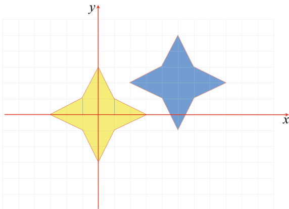
Fig. 15.1 The blue shape is the translated yellow shape
