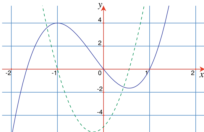
Fig. 16.16 Graph of y = 3x^3 + 2x^2 - 5x and its derivative \frac{dy}{dx} = 9x^2 + 4x - 5 (dashed)
