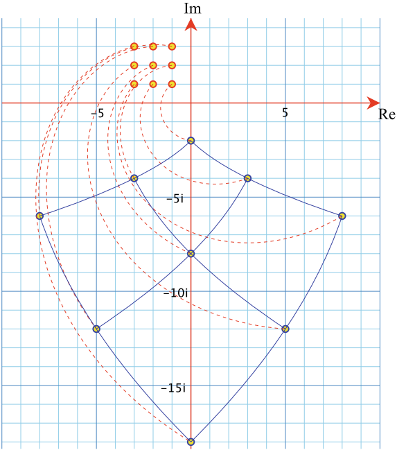
Fig. 13.14 The trajectories of nine complex numbers in the second quadrant, when squared
