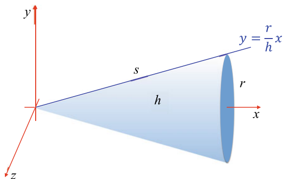
Fig. 19.3 Computing the volume of a right cone
