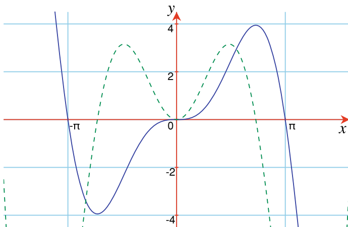
Fig. 16.23 Graph of y = x^2 \sin x and its derivative, \frac{dy}{dx} = x^2 \cos x + 2x \sin x (dashed)
