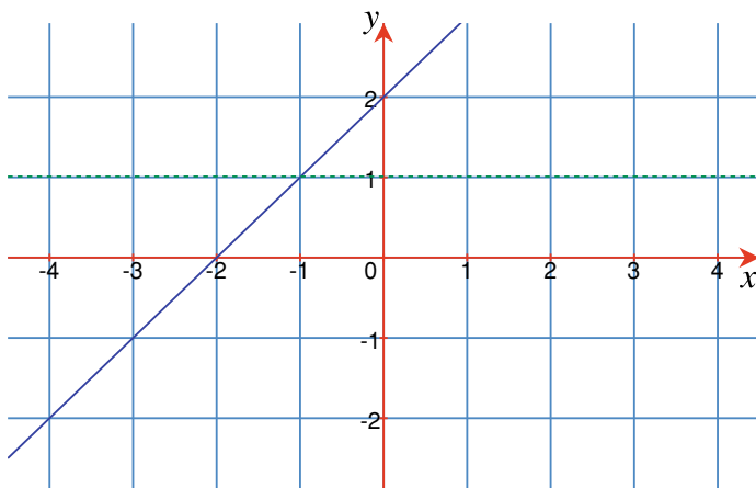
Fig. 16.7 Graph of y = (x^2 + 3)(x + 2)/(x^2 + 3) and its derivative, \frac{dy}{dx} = 1 (dashed)
