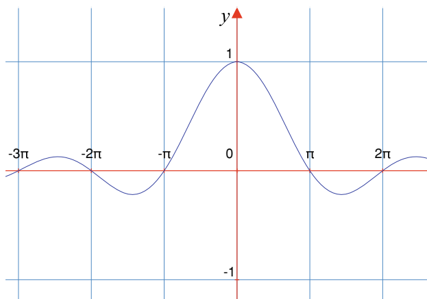
Fig. A.1 Graph of (\sin \theta)/\theta
