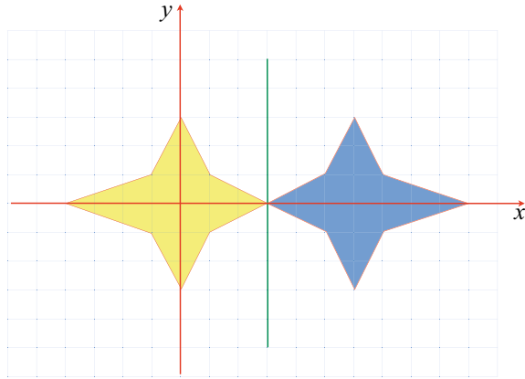
Fig. 15.4 Reflecting a shape about the line x = 3
