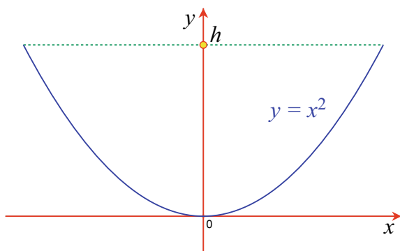
Fig. 19.9 A parabola, which when rotated about the y -axis creates a paraboloid
