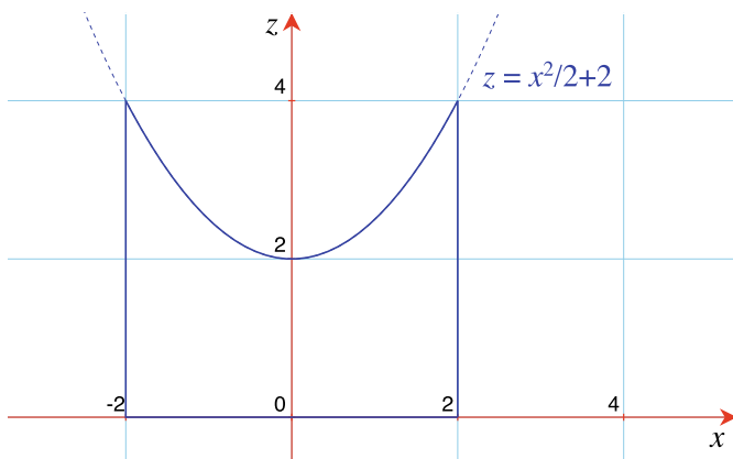
Fig. 19.22 A cross-section of parabola intersecting a cylinder
