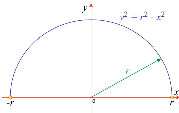
Fig. 19.6 A semi-circle used to form a sphere
