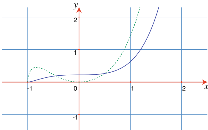
Fig. 17.18 The graphs of y = x^2\sqrt{x^3+1} (dashed) and y = \frac{2}{9}(x^3+1)^{\frac{3}{2}}
