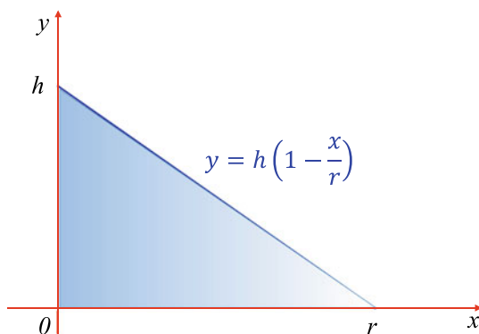
Fig. 19.14 The geometry used to create a right cone
