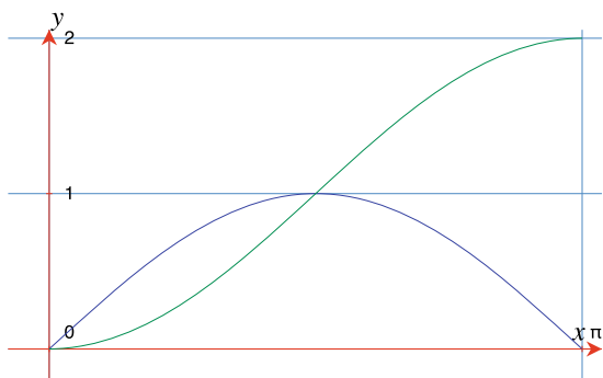
Fig. 18.12 The accumulated area of the sine wave \sin x for x \in [0, \pi]
