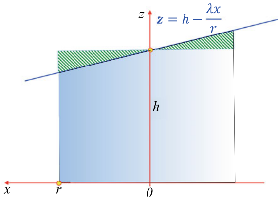
Fig. 19.21 Cross section of a cylinder and intersecting plane
