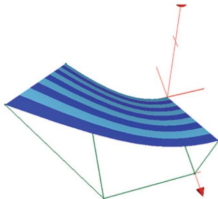
Fig. 19.20 An object with a curved top
