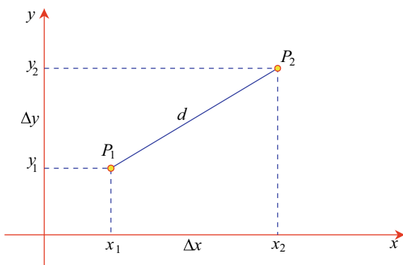
Fig. 10.4 Calculating the distance between two points
