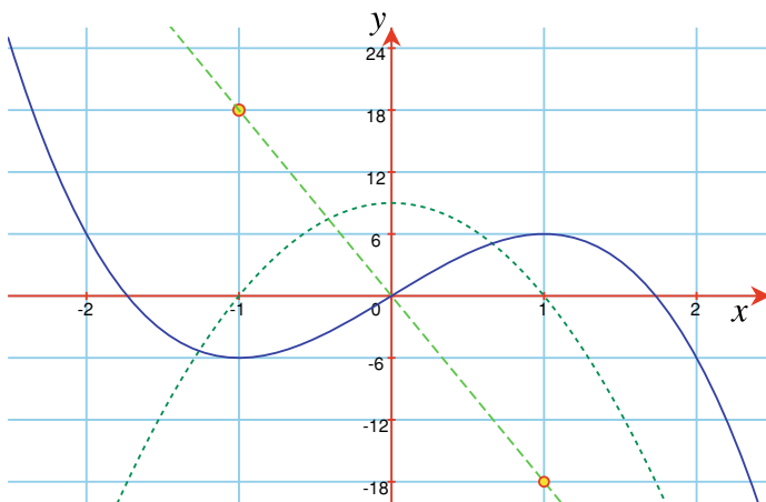
Fig. 16.24 Graph of y = -3x^3 + 9x , its first derivative, \frac{dy}{dx} = -9x^2 + 9 (short dashes) and its second derivative y = -18x (long dashes)
