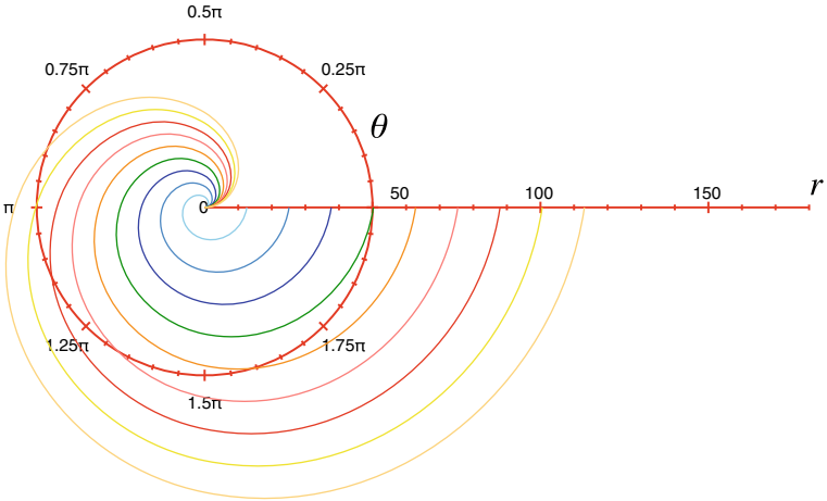
Fig. 10.8 Nine Archimedean spirals
