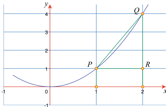
Fig. 16.1 Sketch of f(x) = x^2
