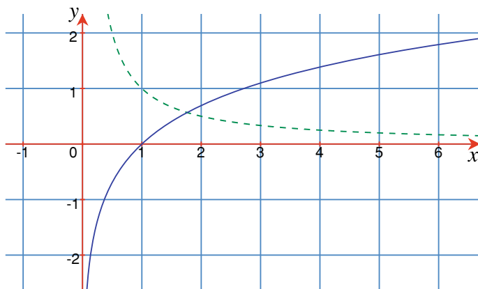
Fig. 16.9 Graph of y = \ln x and its derivative, \frac{dy}{dx} = \frac{1}{x} (dashed)
