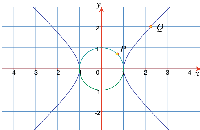
Fig. 16.15 Graphs of the unit circle x^2 + y^2 = 1 and the hyperbola x^2 - y^2 = 1
