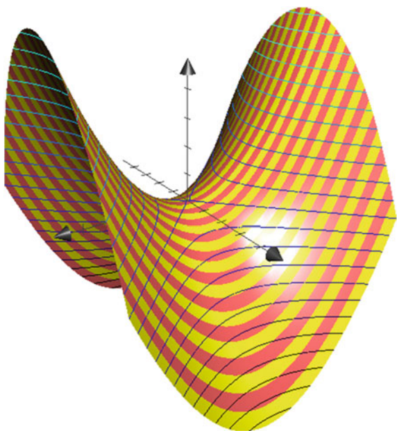
Fig. 16.21 \frac{\partial z}{\partial x} describes the slopes of these contour lines
