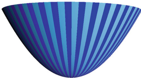
Fig. 19.10 A paraboloid
