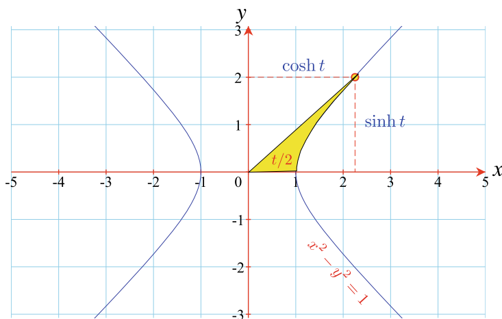
Fig. 13.18 The hyperbolic functions
