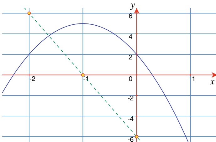
Fig. 16.18 A function containing a local maximum, and its first derivative (dashed)
