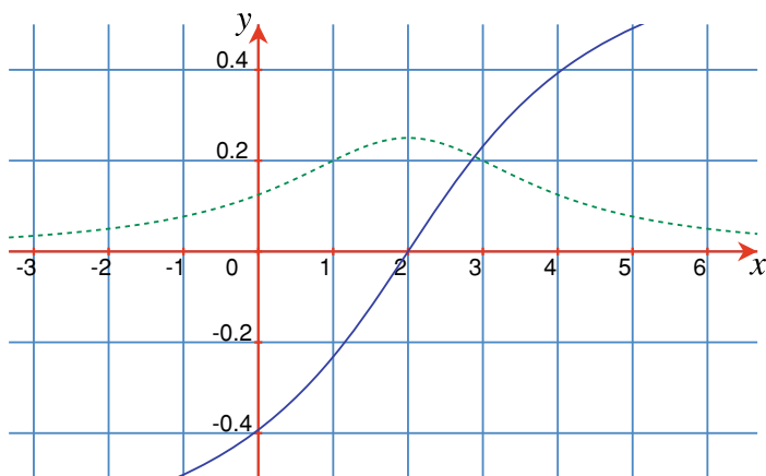
Fig. 17.9 The graphs of y = 1/(x^2 - 4x + 8) (dashed) and y = (\arctan \frac{x-2}{2})/2
