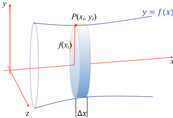
Fig. 19.1 Dividing a volume of revolution into small disks
