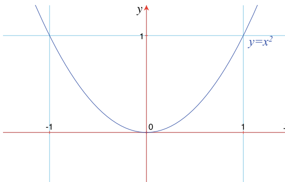
Fig. 18.25 A parabola to be rotated about the y -axis
