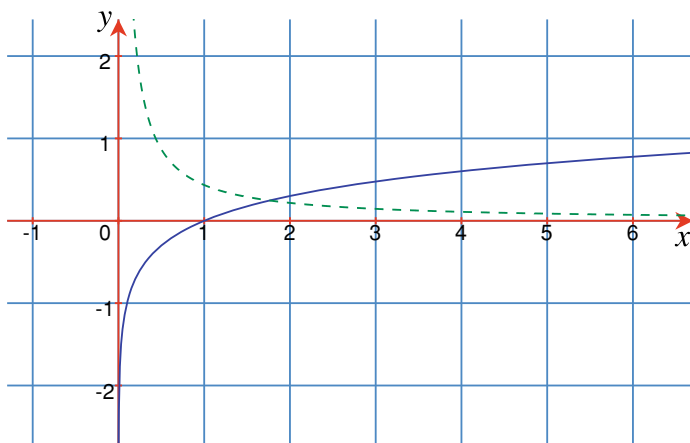
Fig. 16.10 Graph of y = \log_{10} x and its derivative, \frac{dy}{dx} \approx \frac{0.4343}{x} (dashed)
