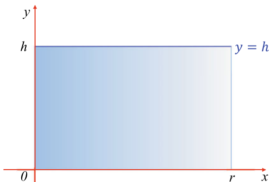
Fig. 19.13 The geometry used to create a cylinder
