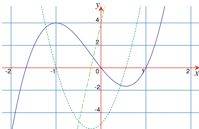
Fig. 16.17 Graph of y = 3x^3 + 2x^2 - 5x , its first derivative \frac{dy}{dx} = 9x^2 + 4x - 5 (short dashes) and its second derivative \frac{d^2y}{dx^2} = 18x + 4 (long dashes)
