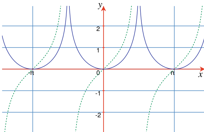
Fig. 17.22 The graphs of y = \sin x / \cos x (dashed) and y = \ln |\sec x|
