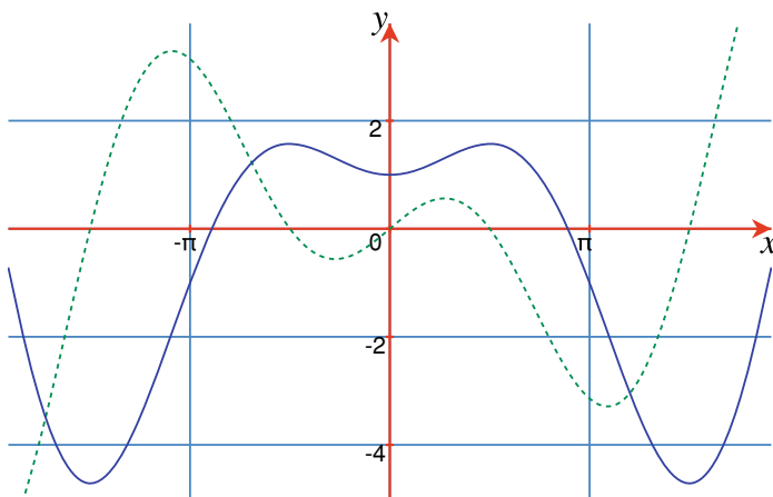
Fig. 17.24 The graphs of y = x \cos x (dashed) and y = x \sin x + \cos x
