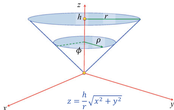
Fig. 19.26 A cone with cylindrical coordinates
