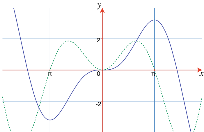
Fig. 17.14 The graphs of y = x \sin x (dashed) and y = -x \cos x + \sin x
