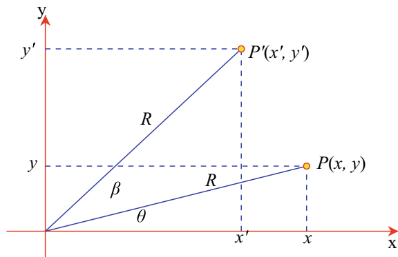
Fig. 15.6 Rotating a point through an angle \beta
