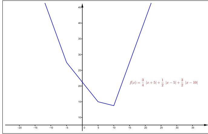
Figure 5.4: A nondifferential convex function.
