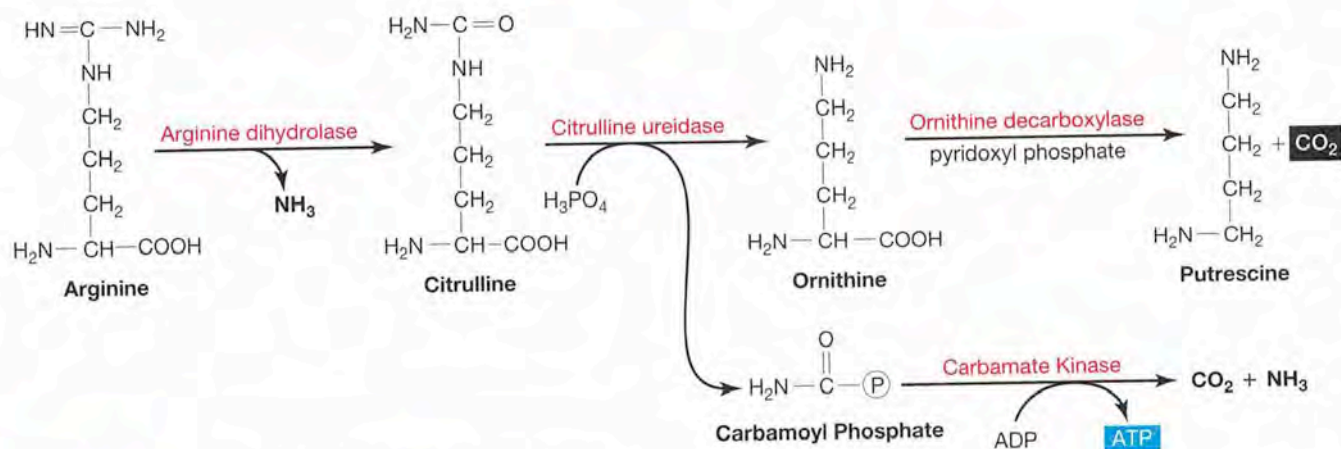
FIGURE 33.7 Arginine Dihydrolase System • In addition to decarboxylation, arginine may also be catabolized by a dihydrolase enzyme with the production of ornithine, \text{NH}_3 , and \text{CO}_2 . In ornithine decarboxylase-positive organisms, the ornithine is further degraded into putrescine and \text{CO}_2 . The example shown here is a dihydrolase system of Pseudomonas putida in which ATP synthesis occurs. Regardless of the specifics, the arginine dihydrolase pathway is indistinguishable from the arginine decarboxylase pathway because both produce alkaline end products.
