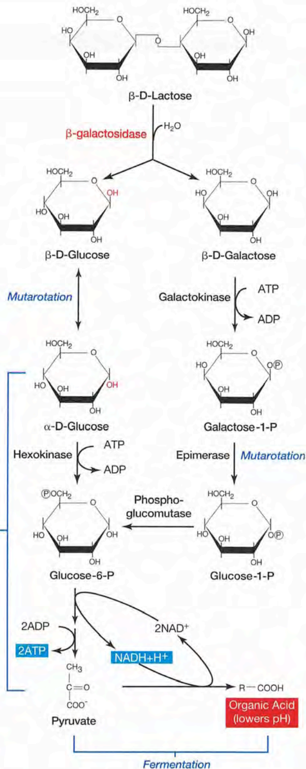
FIGURE 23.1 Lactose Fermentation with Acid End Products • A key end product of lactose fermentation is an organic acid (red box in the figure). That acid is detected by the neutral red pH indicator in MAC agar. For simplicity, only the relevant parts of glycolysis are shown. See Appendix A, Figure A.2 for details.
