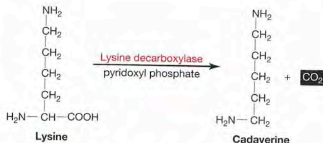
FIGURE 33.4 Lysine Decarboxylation • Decarboxylation of the amino acid lysine produces cadaverine and \text{CO}_2 .
