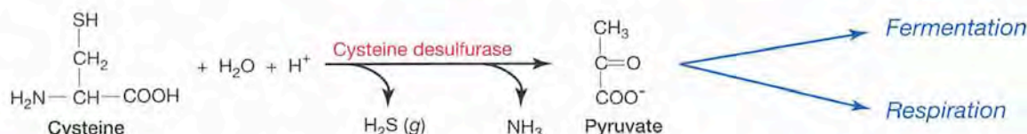
FIGURE 36.1 Sulfur Reduction: H_2S Production from Cysteine Hydrolysis (Cysteine Desulfurase Reaction) • In putrefaction, cysteine desulfurase catalyzes the hydrolysis of the amino acid cysteine with the production of pyruvate, ammonia ( NH_3 ), and hydrogen sulfide ( H_2S ).
