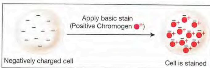
FIGURE 11.3 Chemistry of Basic Stains • Basic stains have a positively charged chromogen, which readily associates with the negatively charged bacterial cell to colorize it.
