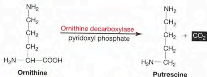
FIGURE 33.5 Ornithine Decarboxylation • Decarboxylation of the amino acid ornithine produces putrescine and \text{CO}_2 .
