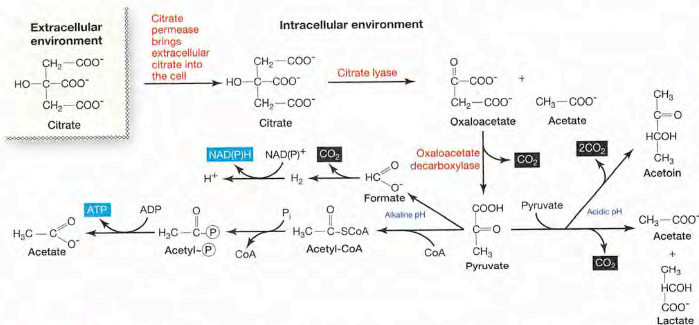
FIGURE 32.1 Citrate Chemistry • Citrate permease imports citrate into the cell. From there, citrate lyase converts citrate into oxaloacetate and acetate. Next, the enzyme oxaloacetate decarboxylase performs a decarboxylation reaction in which \text{CO}_2 is removed from oxaloacetate thereby forming pyruvate. The resulting pyruvate can be converted to a variety of products depending on the pH of the cell's environment and the enzymes the cell possesses. One option, the formate/acetyl-CoA pathway shown in detail to the left, produces the useful compounds ATP and NADH/NADPH.
