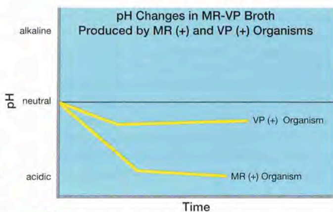
FIGURE 28.3 Mixed Acid Versus Butanediol Fermentation and the Effects on MR-VP Media pH • The MR-VP test differentiates between organisms that perform mixed acid fermentation and those that conduct butanediol fermentation. Mixed acid fermentation lowers the test broth's pH due to the abundance of acidic end products that are made. In contrast, organisms that perform butanediol fermentation make primarily neutral end products.
