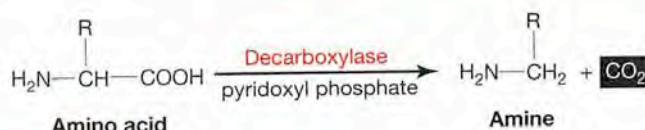
FIGURE 33.2 Amino Acid Decarboxylation • Removal of an amino acid's carboxyl group results in the formation of an amine and carbon dioxide.
