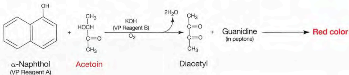
FIGURE 28.6 Voges-Proskauer Test Indicator Reaction • Adding potassium hydroxide (KOH) raises the sample's pH and promotes the oxidation of acetoin to form diacetyl. In this reaction, 5% \alpha -naphthol enhances the development of the red color seen in a positive test result.
