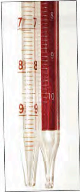
FIGURE C.4 Two Types of Pipettes • Two pipette styles—the serological pipette (left) and the Mohr pipette (right)—are used in microbiology. A serological pipette is calibrated to deliver (TD) its volume by completely draining it and blowing out the last drop. The tip of a Mohr pipette is not graduated, so fluid flow must be stopped at a calibration line. Stopping the fluid beyond the last line on a Mohr pipette results in an unknown volume being dispensed.
