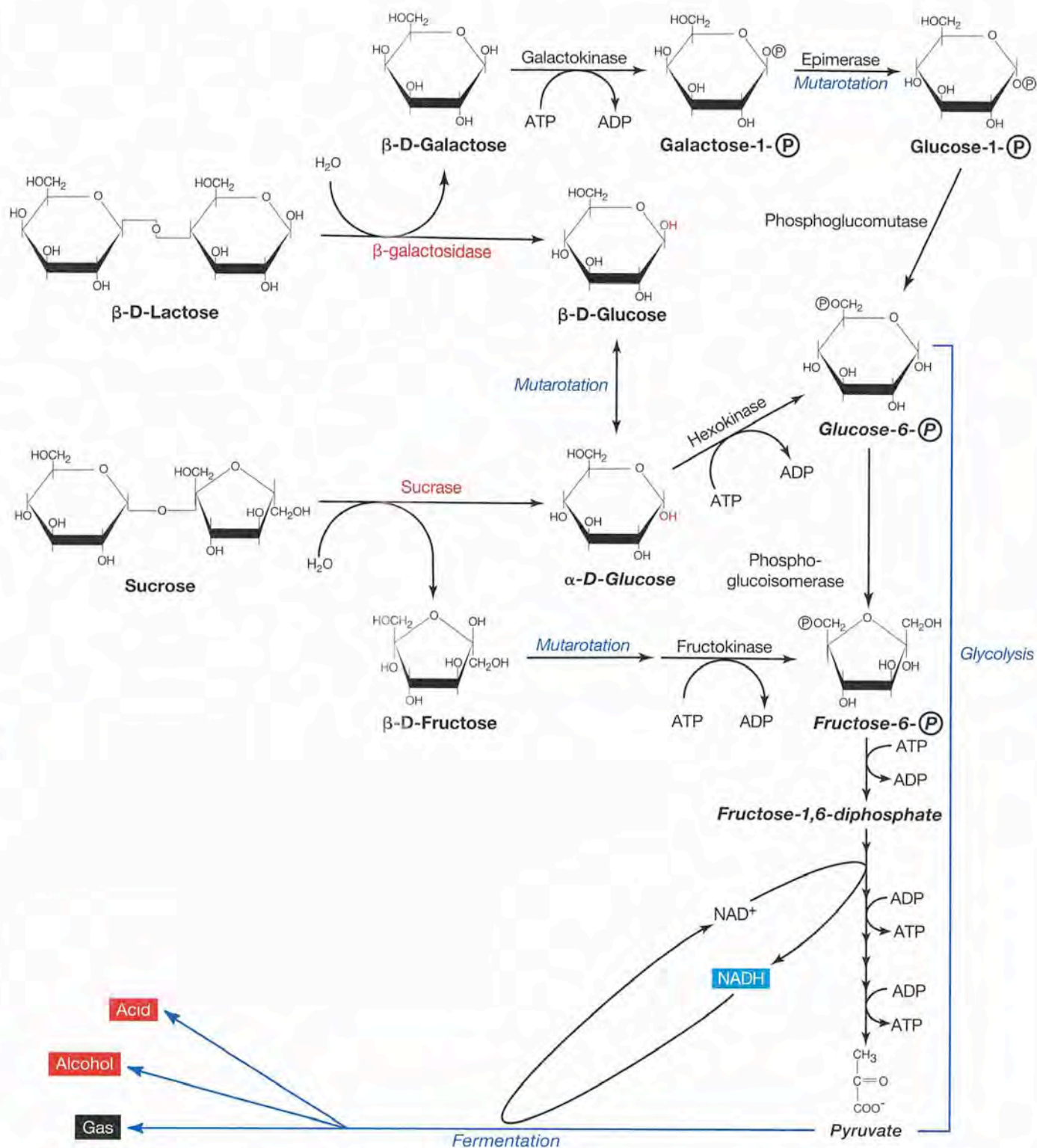
FIGURE 27.1 Fermentation of Glucose and the Disaccharides Lactose and Sucrose • Enzymes hydrolyze the disaccharides lactose and sucrose to release monosaccharides. These monosaccharides are then funneled into glycolysis as the initial stage in fermentation. The enzyme \beta -galactosidase hydrolyzes lactose into glucose and galactose whereas sucrase hydrolyzes sucrose to release glucose and fructose.
