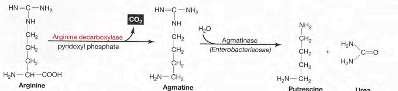
FIGURE 33.6 Arginine Decarboxylation • Decarboxylation of the amino acid arginine produces the amine agmatine. Members of Enterobacteriaceae are capable of degrading agmatine into putrescine and urea. Those strains with urease (see Ex. 35) can further break down the urea into ammonia and carbon dioxide. Thus, the end products of arginine catabolism are carbon dioxide, putrescine, and urea, or (in the presence of urease) carbon dioxide, putrescine, and ammonia.
