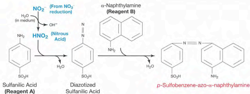
FIGURE 31.4 Indicator Reaction for Nitrate Reduction to Nitrite • If nitrate is reduced to nitrite, nitrous acid ( \text{HNO}_2 ) will form in the medium. Nitrous acid then reacts with sulfanilic acid (Reagent A) to form diazotized sulfanilic acid, which reacts with the \alpha -naphthylamine (Reagent B) to form p -sulfobenzene-azo- \alpha -naphthylamine, which is red. Thus, a red color indicates the presence of nitrite and is considered a positive result for nitrate reduction to nitrite.
