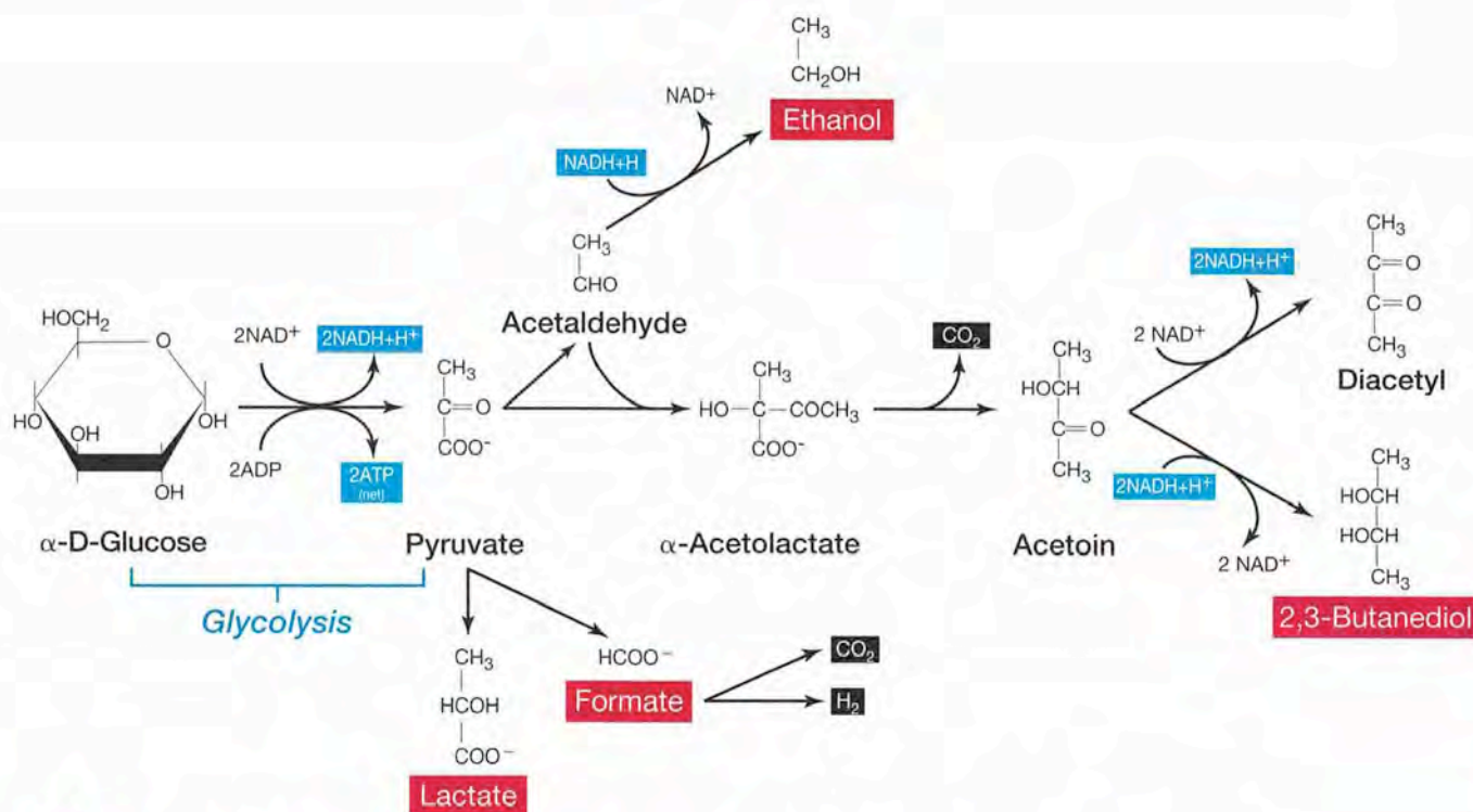
FIGURE 28.2 Butanediol Fermentation Pathway • Butanediol fermentation primarily produces the neutral molecules 2,3-butanediol and ethanol.
