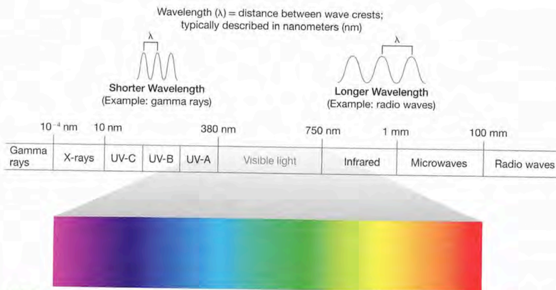
FIGURE 42.1 Electromagnetic Spectrum • Gamma rays have the shortest and highest energy wavelengths ( \lambda less than 10 -4 nm). In contrast, radio waves have long wavelengths that can be 1 kilometer or longer. Between about 100 nm and 380 nm (just shorter than visible light) is the portion known as ultraviolet light.
