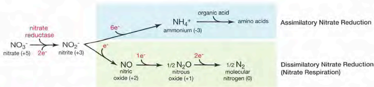
FIGURE 31.1 Possible End Products of Nitrate Reduction • In the presence of nitrate reductase, nitrate ( \text{NO}_3^- ) undergoes a single reduction to form nitrite ( \text{NO}_2^- ). Nitrite can then be further reduced via dissimilatory nitrate reduction or assimilatory nitrification. In each compound, nitrogen's oxidation state is shown in parentheses. Notice that as electrons are added, nitrogen's oxidation state decreases.
