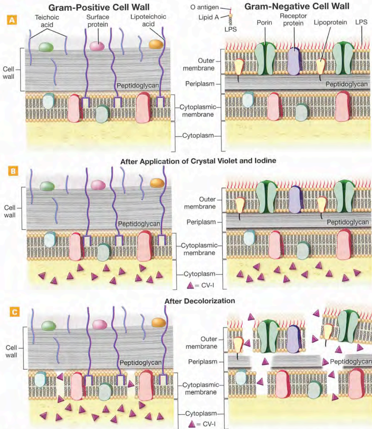
FIGURE 13.3 Chemistry of the Gram Stain • The Gram stain differentiates between Gram-positive and Gram-negative bacteria based on cell wall features. (A) As compared to the Gram-positive bacterial cell wall (left), the Gram-negative wall (right) has a thin peptidoglycan layer and more lipid (due to the outer membrane). (B) Relatively large crystal violet–iodine complexes (purple triangles) form in the cytoplasm of both Gram-positive and Gram-negative cells. (C) The thicker Gram-positive peptidoglycan layer dehydrates when decolorizer is added, trapping the crystal violet–iodine complexes. The lipid in the Gram-negative cell wall is dissolved by the decolorizer and the thinner peptidoglycan is incapable of preventing extraction of the crystal violet–iodine complex.
